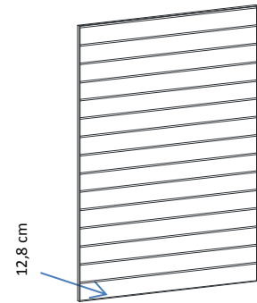
PR-24 Paneelrahmen 1
